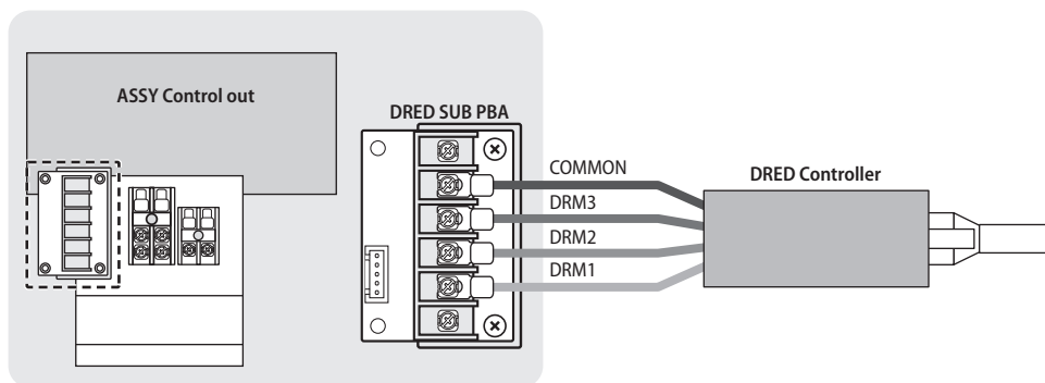
Outdoor unit
